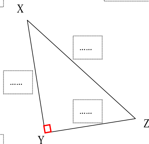
Triangle rectangle
